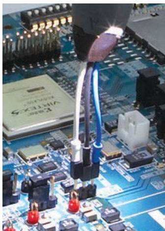
N2750A with socketed tip
