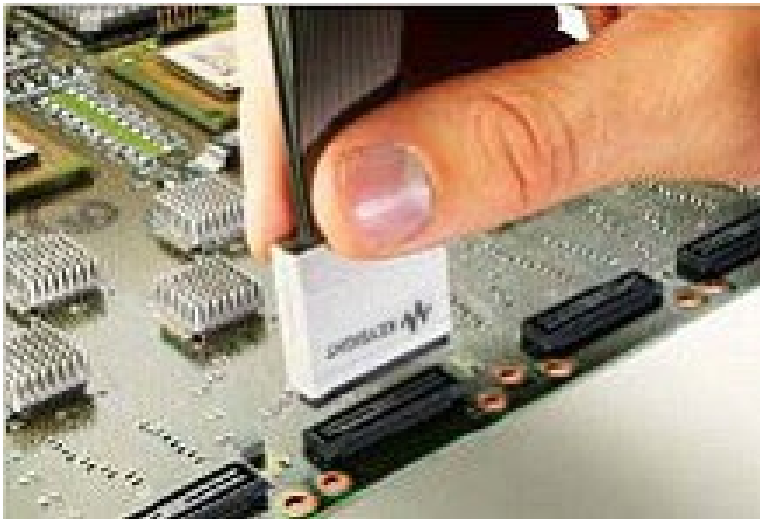
E5385A 34-channel Samtec connector probe
